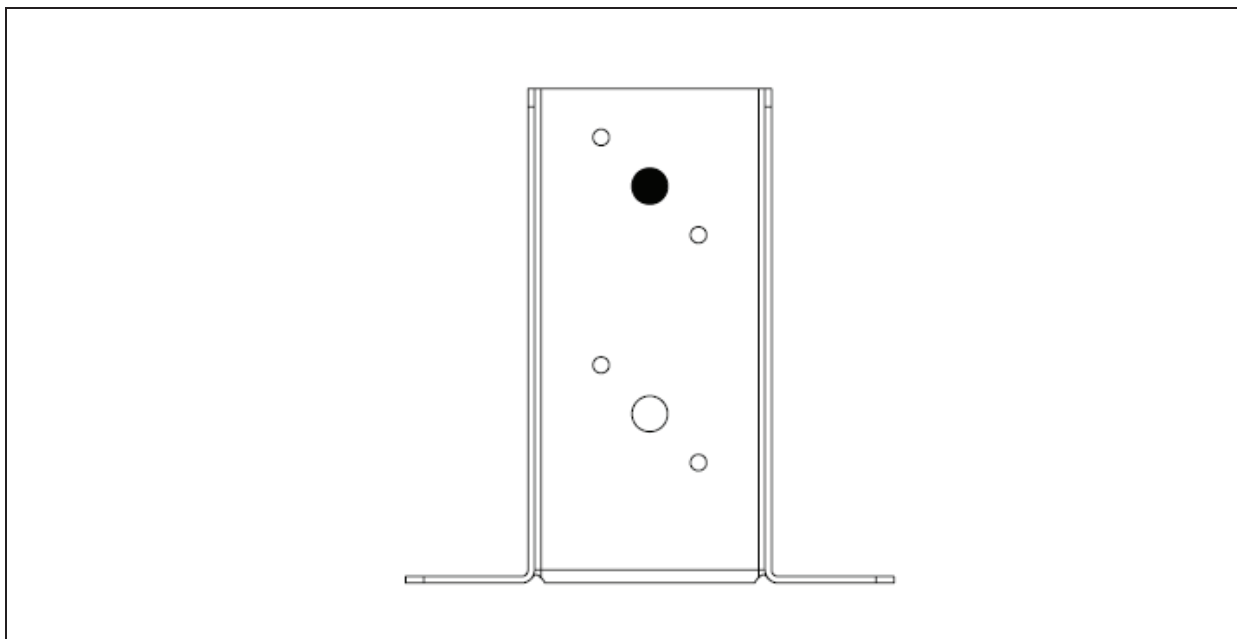
Rysunek 54 Typ PSPDX 45, PSPDX 70, PSPDX 90, PSPDX 100, PSPDX 120, PSPDX 140, PSPDX 150
